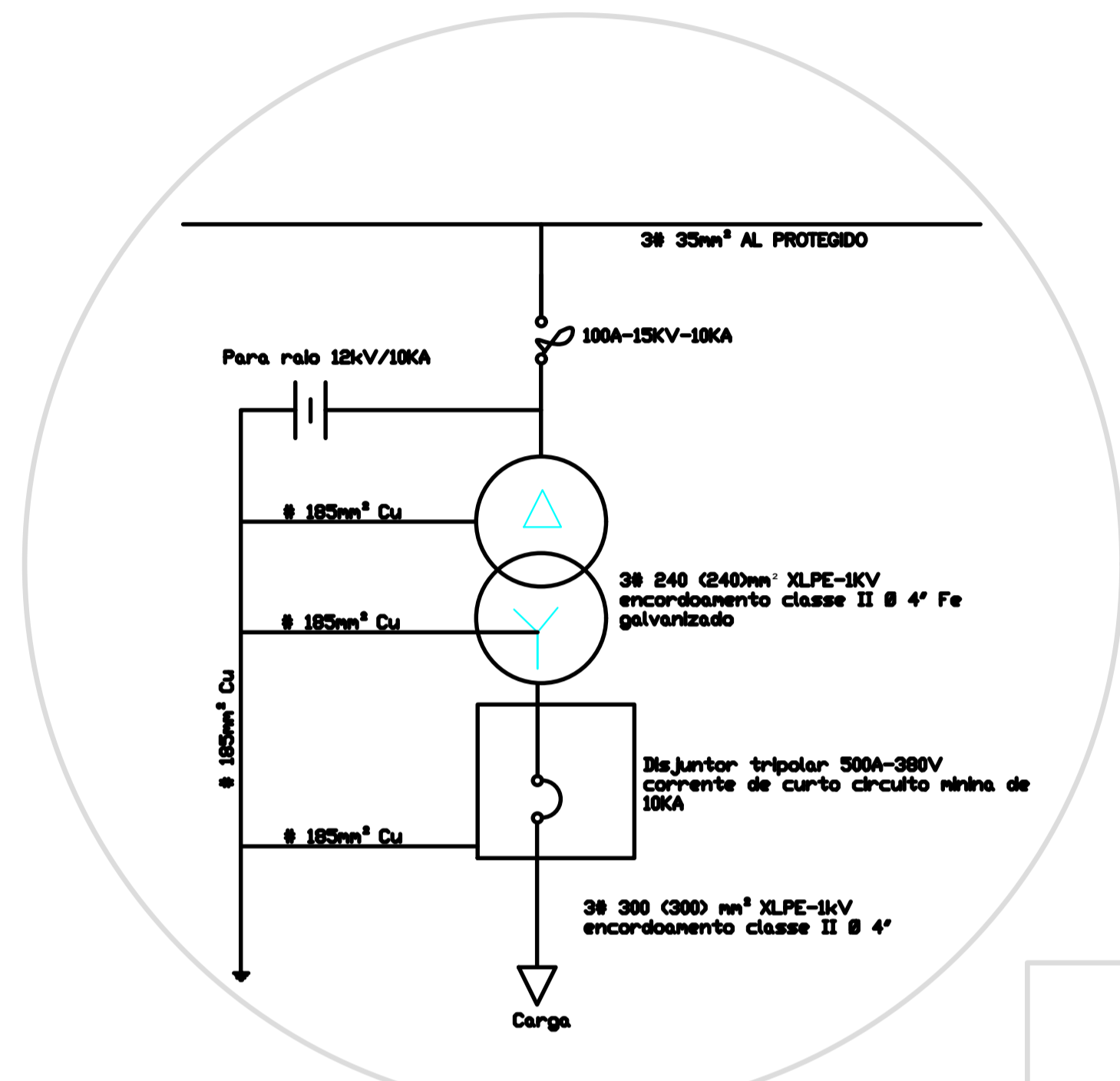
DIAGRAMA UNIFILAR
